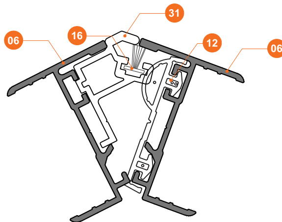
Section of 135° Joining
