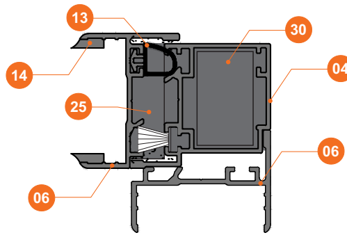
Section of 90° Joining
